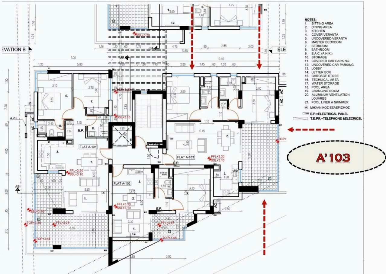
BLOCK A' FIRST FLOOR PLAN
