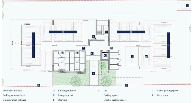
BUILDINGS A & B GROUND FLOOR
