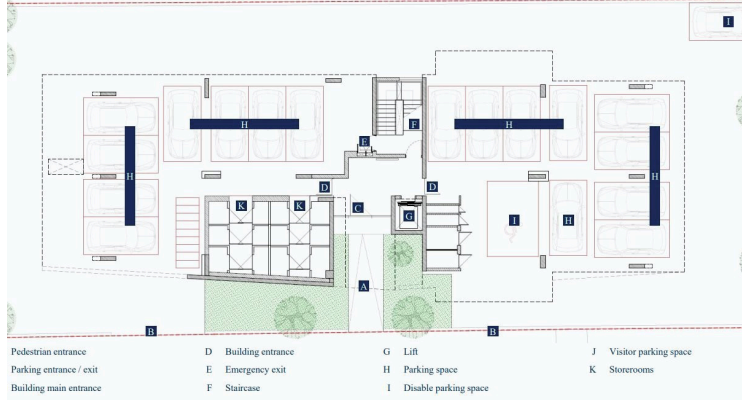
PLANTINGS A & B GROUND FLOOR
