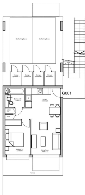
Ground floor Plan 1 Bed Cluster
